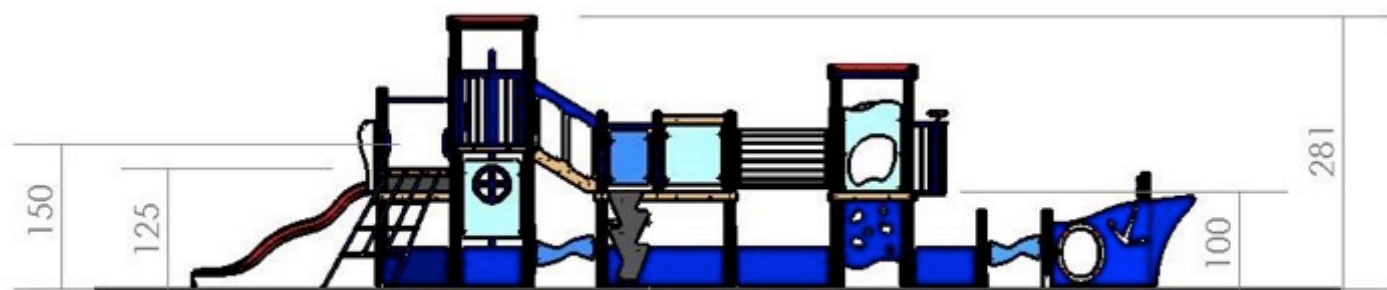
Dimensions of the Equipment and Minimum Space for Placement
